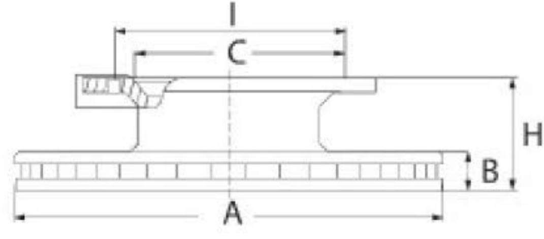
MAN 12.163 ARKA ( REAR ) ABS
