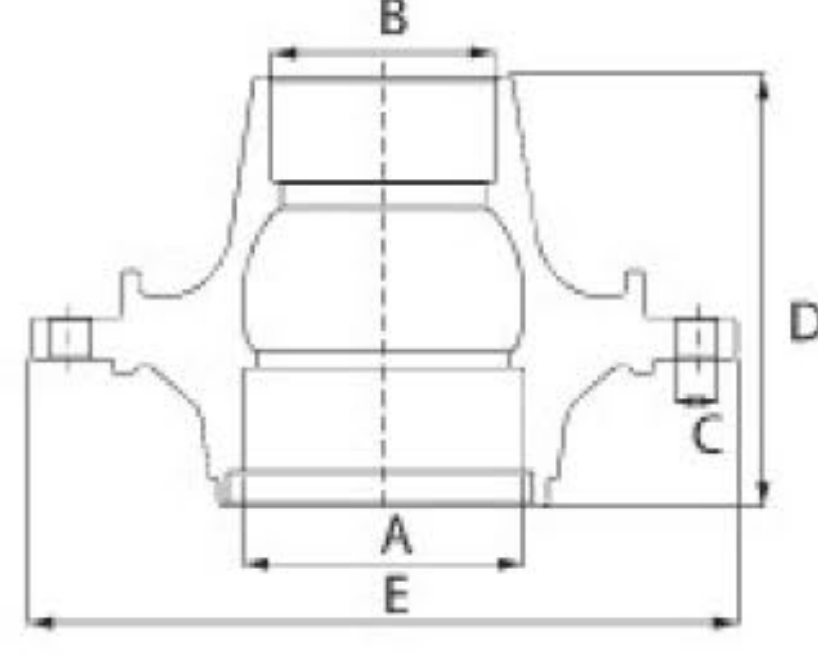
IVECO 50 NC Y.M ÖN PORYA WHEEL HUB / FRONT (NEW MODEL)
