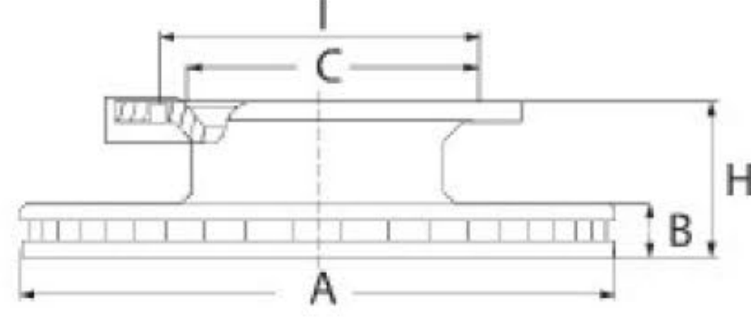
IVECO EUROCARGO 100E 18 (ABS) ARKA
