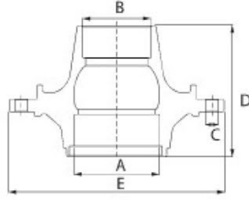
ISUZU NPR ÖN PORYA WHEEL HUB / FRONT
