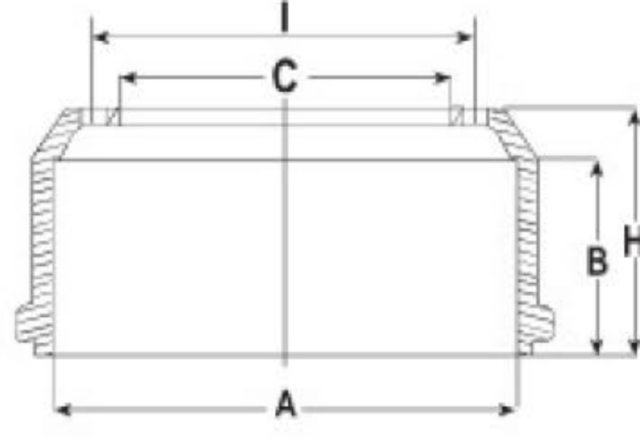
VOLVO F10-F12 ESKİ MODEL (OLD MODEL)
