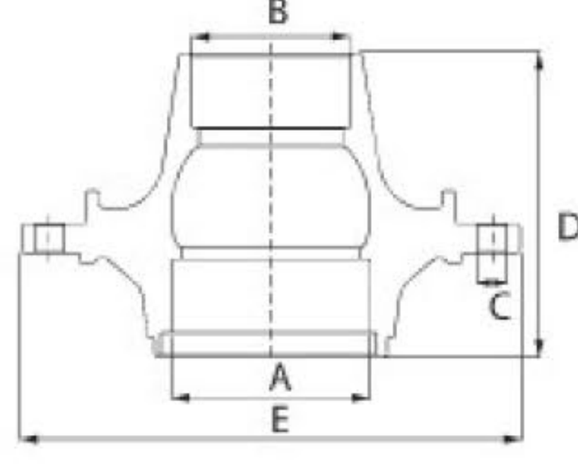
ISUZU NPR 75 ABS ARKA PORYA WHEEL HUB / REAR
