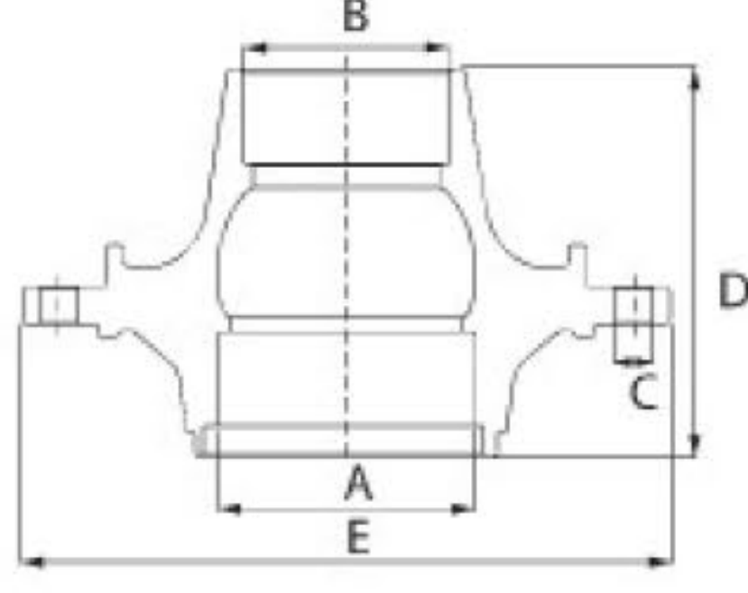
DAF XF-CF ÖN DİSKLİ PORYA (2006 VE SONRASI) WHEEL HUB (FOR BRAKE DISC)
