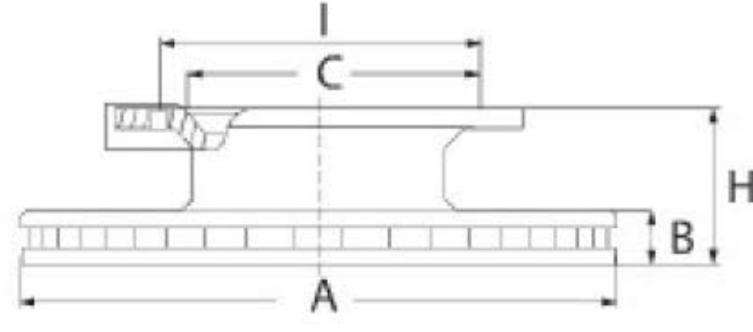
IVECO DAILY 70-C-15 ÖN Y.M. (FRONT / NEW MODEL)
