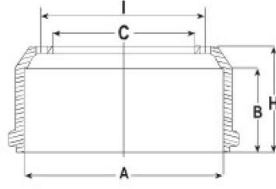
BPW 7.5 CM UZUN KUŞAK (LONG BELT)
