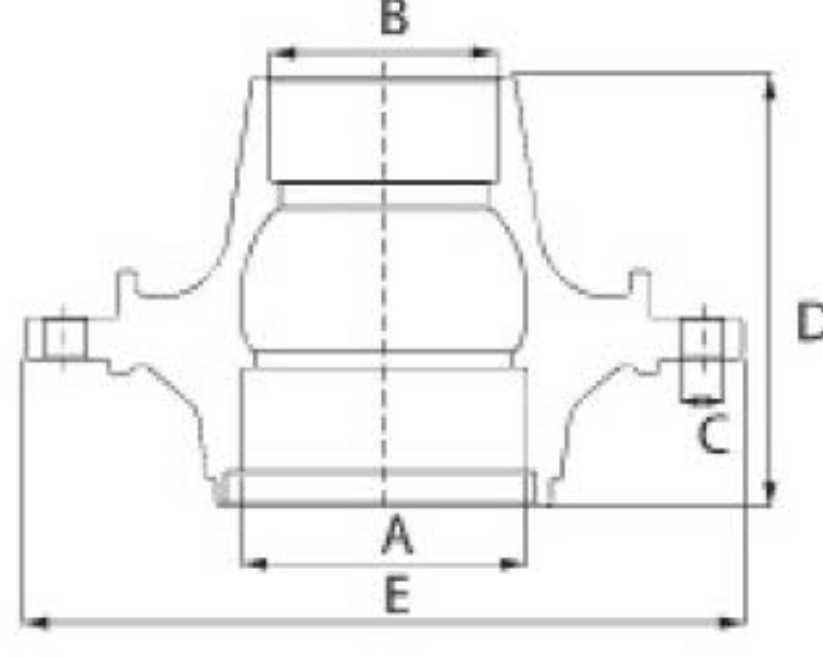
SAF Y.M. PİLOT PORYA DİSKLİ (88'LİK) WHEEL HUB ( NEW MODEL FOR BRAKE DISC)
