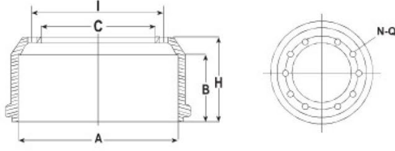
FATİH-BMC 27026 DEV FATİH SOĞUTMALI (COOLED)
