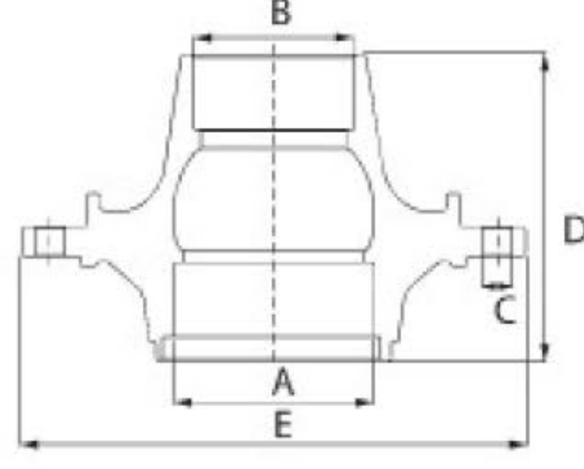
RENAULT 270 ÇEKİCİ PORYA WHEEL HUB / REAR
