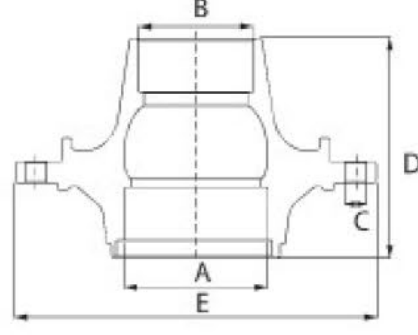
VOLVO FM 9 ÇEKİCİ PORYA WHEEL HUB / REAR
