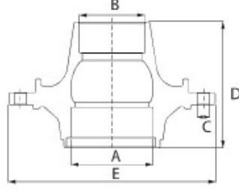
O403 - O404 OTOBÜS DİSKLİ ÖN WHEEL HUB / FRONT (FOR BRAKE DISC)
