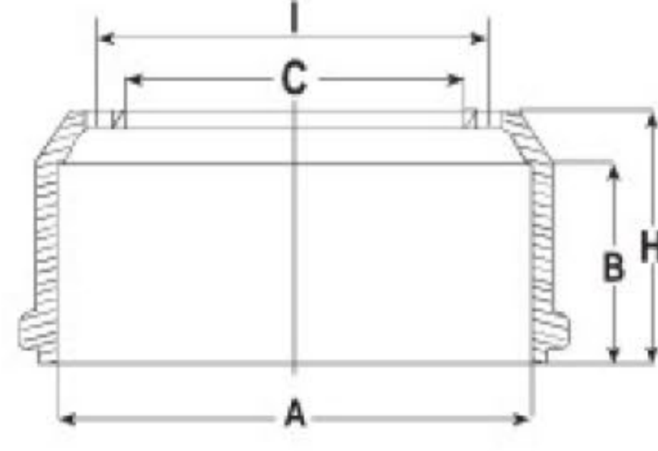
IVECO 50 NC ESKİ MODEL ÖN ( FRONT / OLD MODEL )
