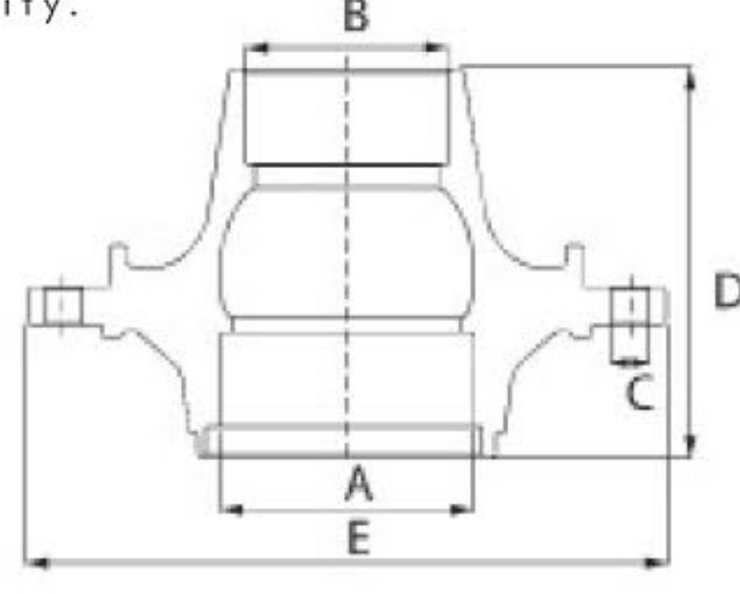
MAN TGA ÖN RULMAN ÜNİTESİ WHEEL HUB / FRONT (FOR BRAKE DISC)
