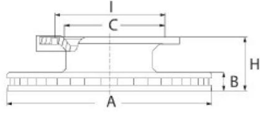
MAN 19.463 SG 90 F 2000 10 DELİK (HOLES)
