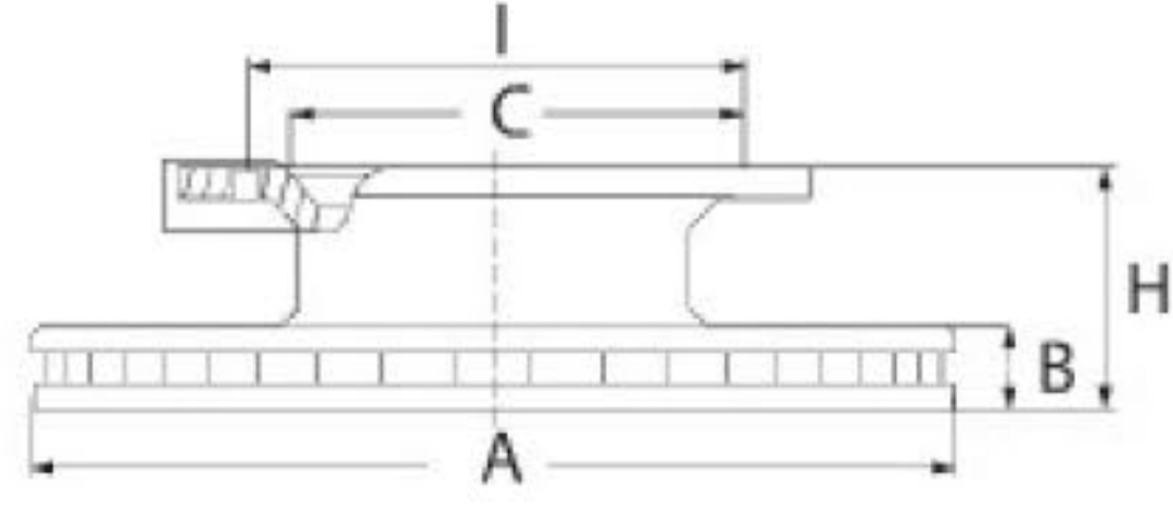
SAF KÜÇÜK 8 DELİK (HOLES)
