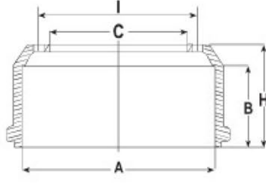
O345 CONECTO EURO 3 SOĞUTMALI (COOLED)
